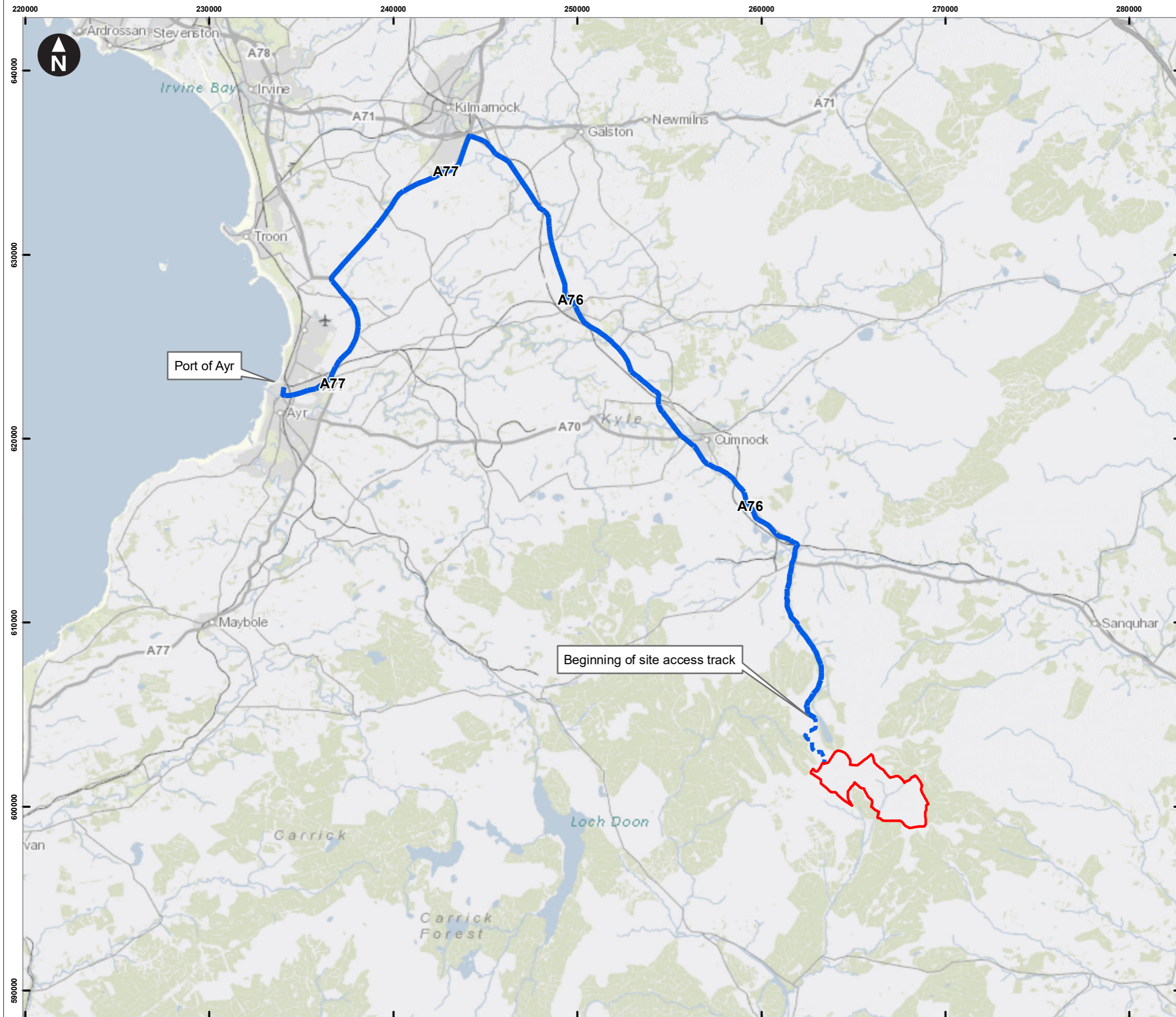
Figure 14.2 Proposed turbine delivery route from the Port of Ayr
