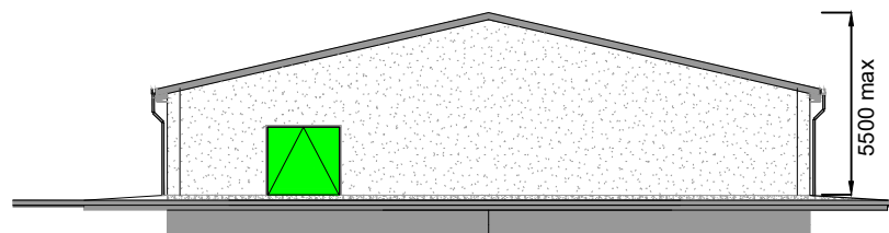
Control Building End Elevation 1 1:250
