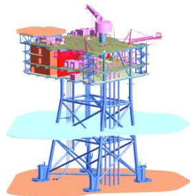
Clipper South Plattform Design
