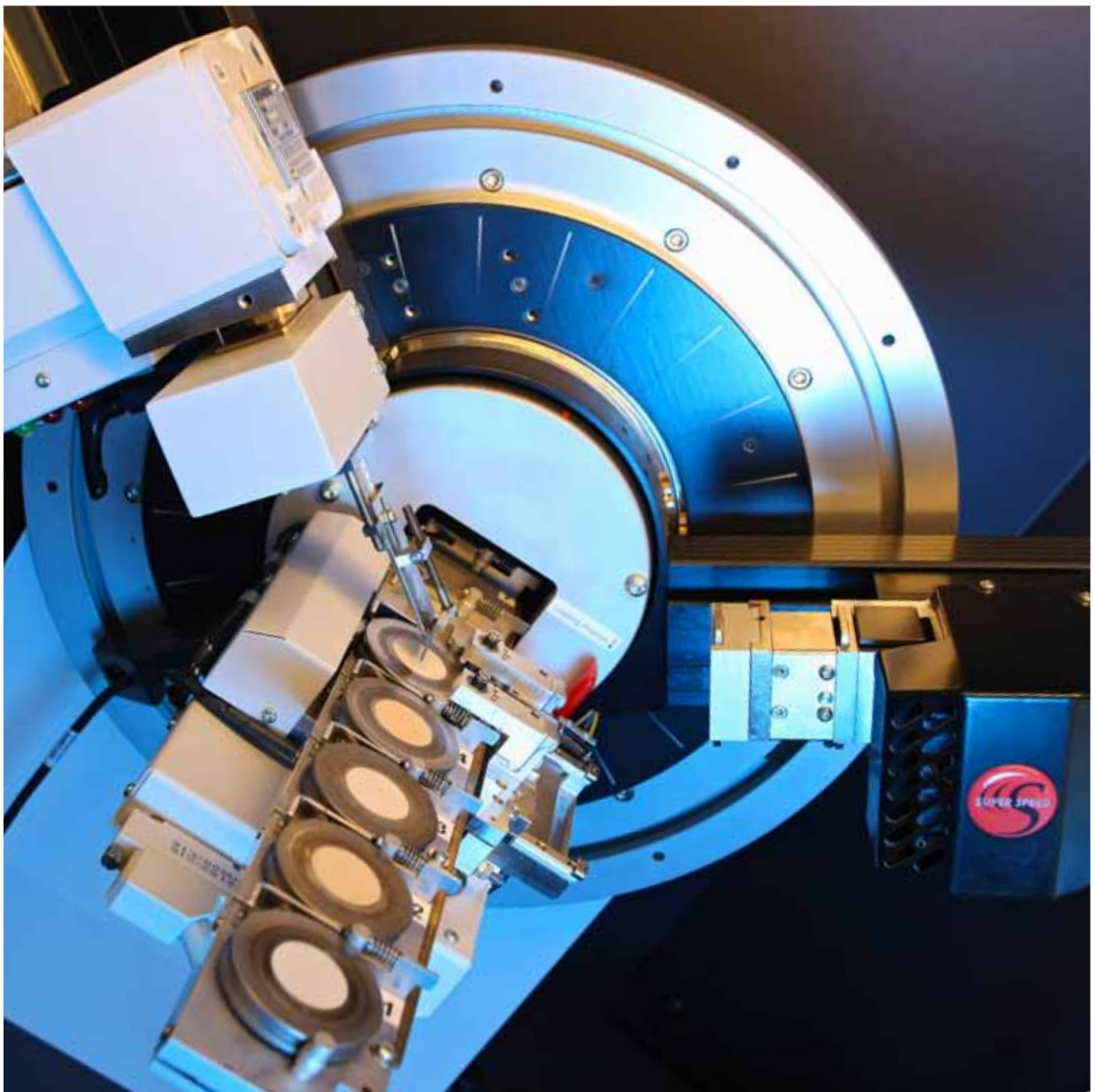
A sample is prepared for analysis under the X-ray diffractometer in the RWE Dea laboratory.
